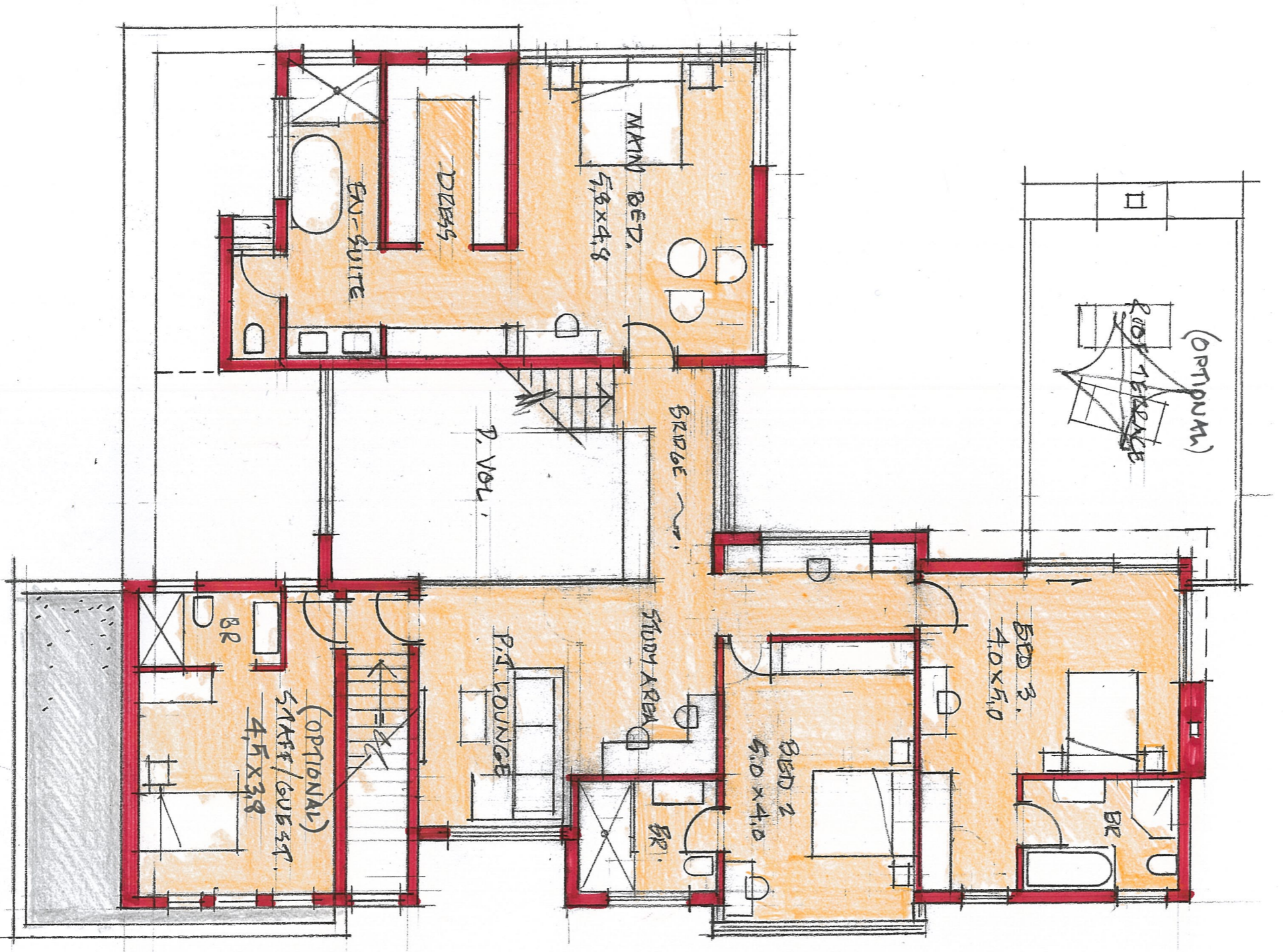
FIRST FLOOR PLAN, (178 m 2 STAFF OPTIONAL 30 m 2 ) "THE LINCOLN"
